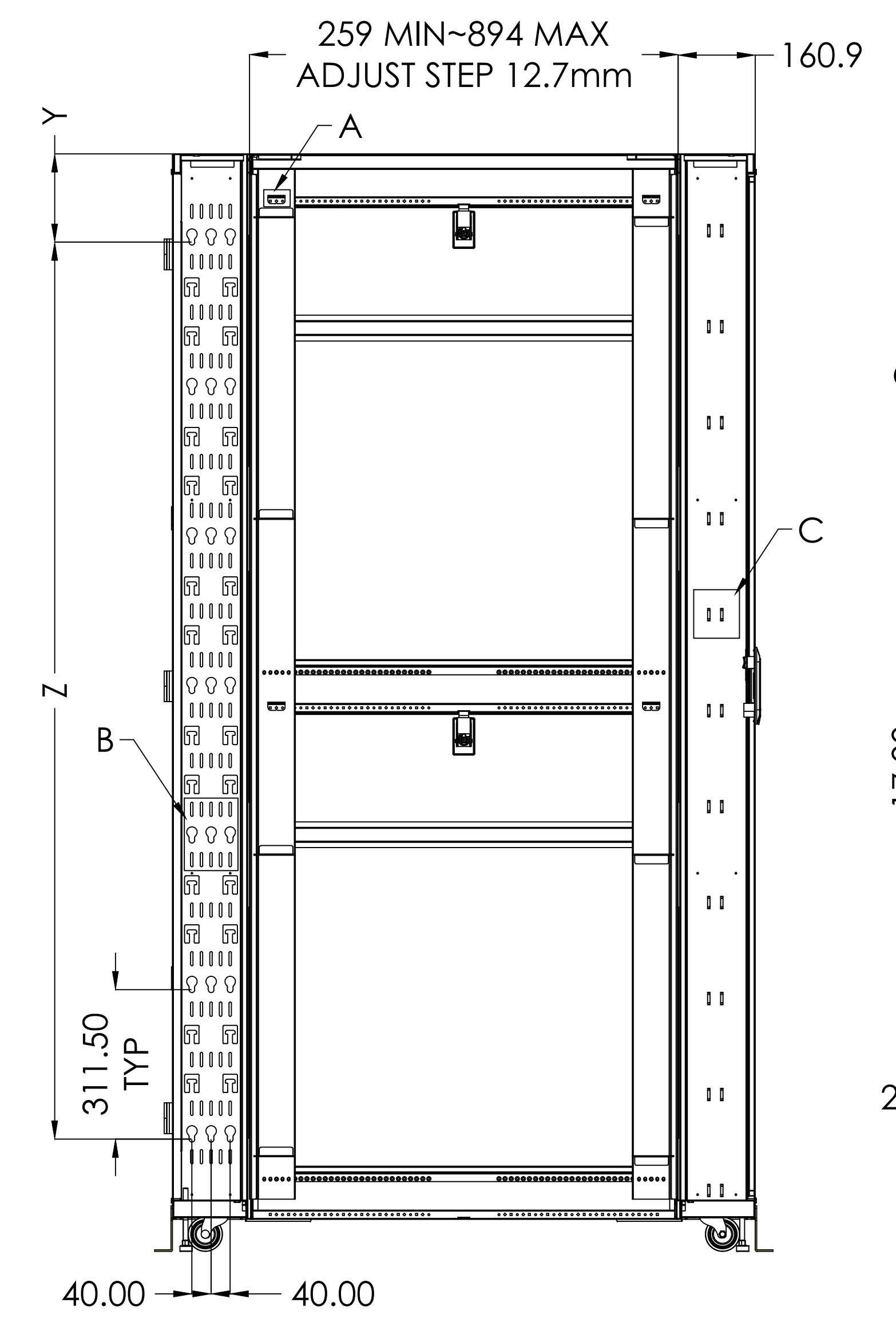
SECTIONAL VIEW C-C
