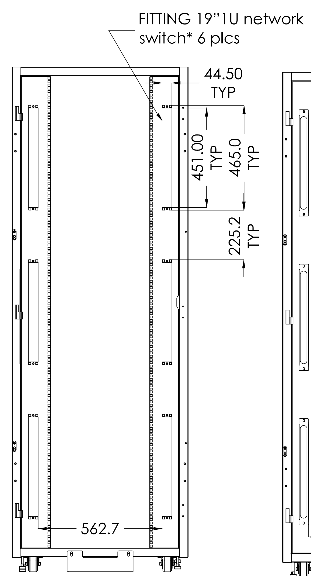
FRONT VIEW (WITHOUT DOORS AND BRUSHES)
