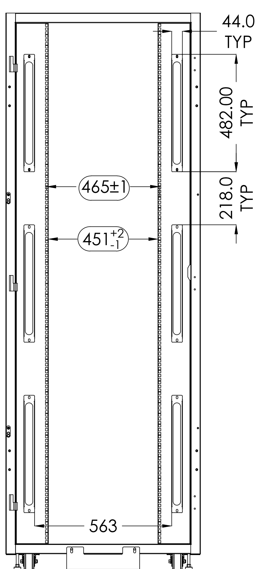
FRONT VIEW (WITHOUT DOORS AND WITH BRUSHES)
