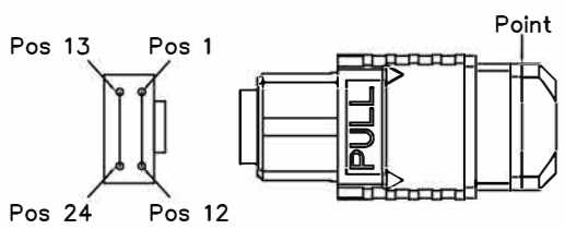
MTP Female Connector A
