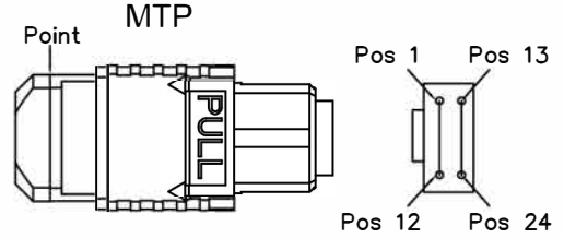
MTP Female Connector B
