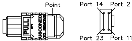
MTP Female Connector
