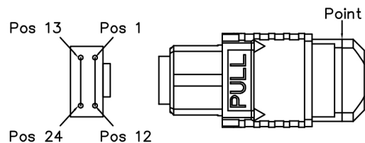
MPO Female Connector A
