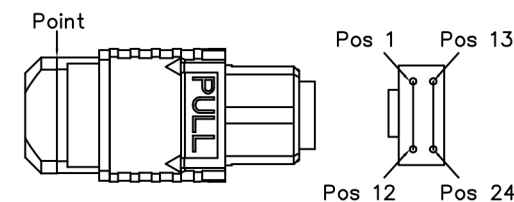
MPO Female Connector B
