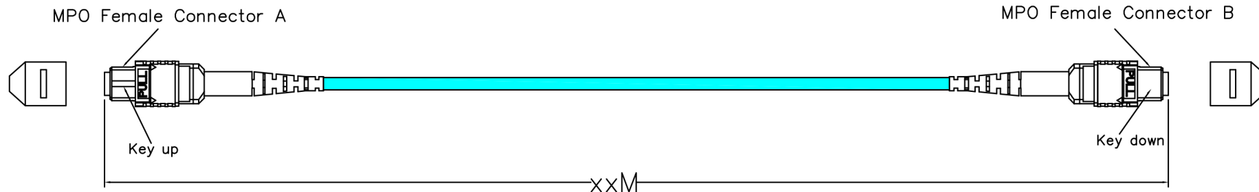
MPO Female Connector A
