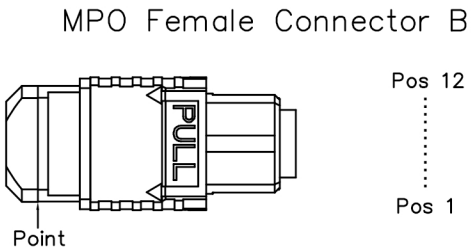
Connector B
