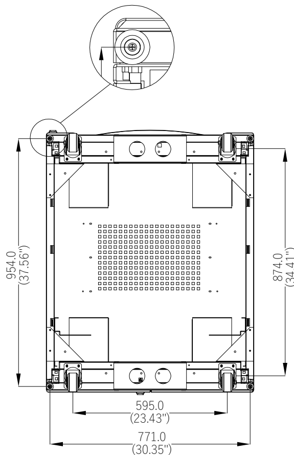
Bottom View
