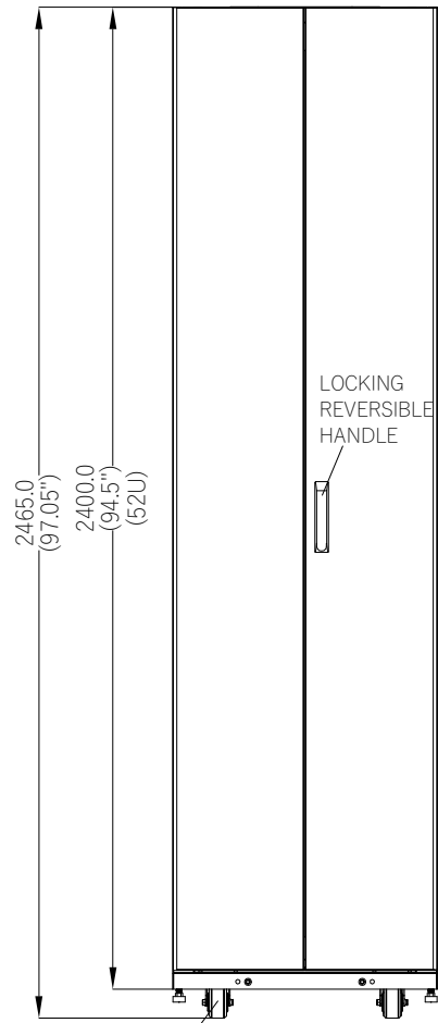
Rear View
