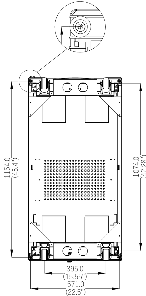
Bottom View
