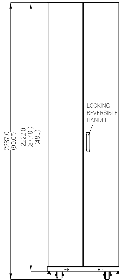
Rear View 3" Heavy Duty Casters
