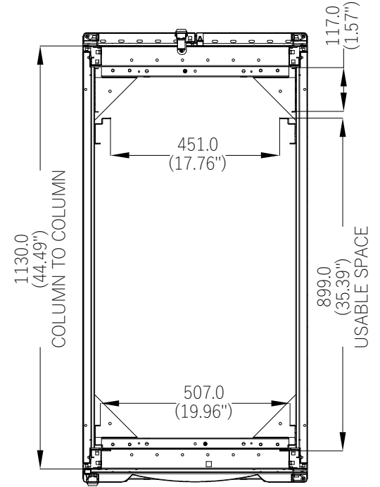
A-A Profile View
