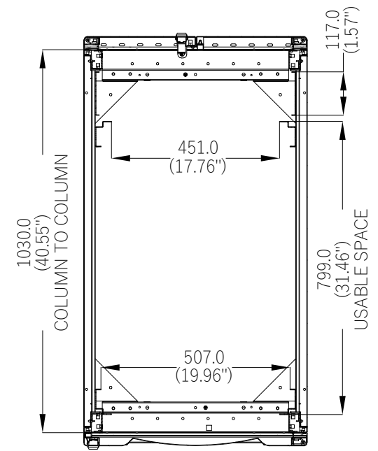
A-A Profile View
