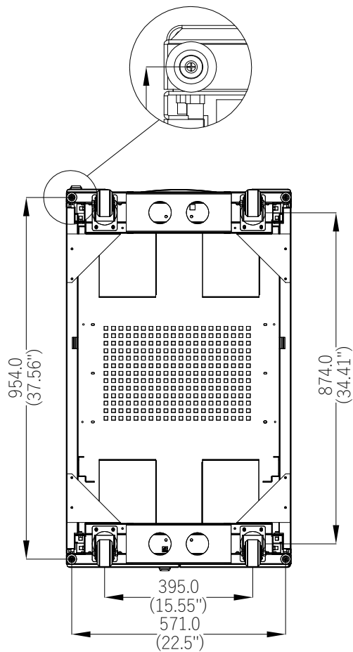
Bottom View
