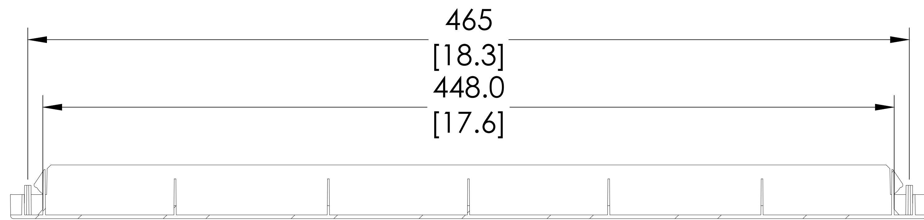
SECTIONAL VIEW A-A
