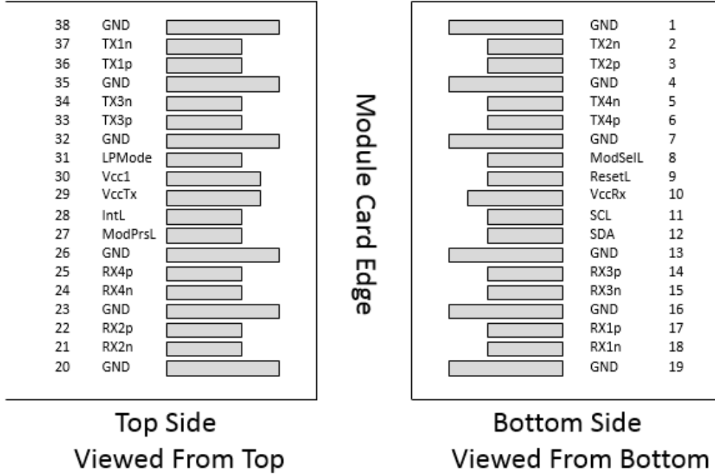
Figure 3. QSFP28 MSA compliant Connector
