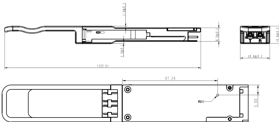
Figure 5. Mechanical Dimensions
