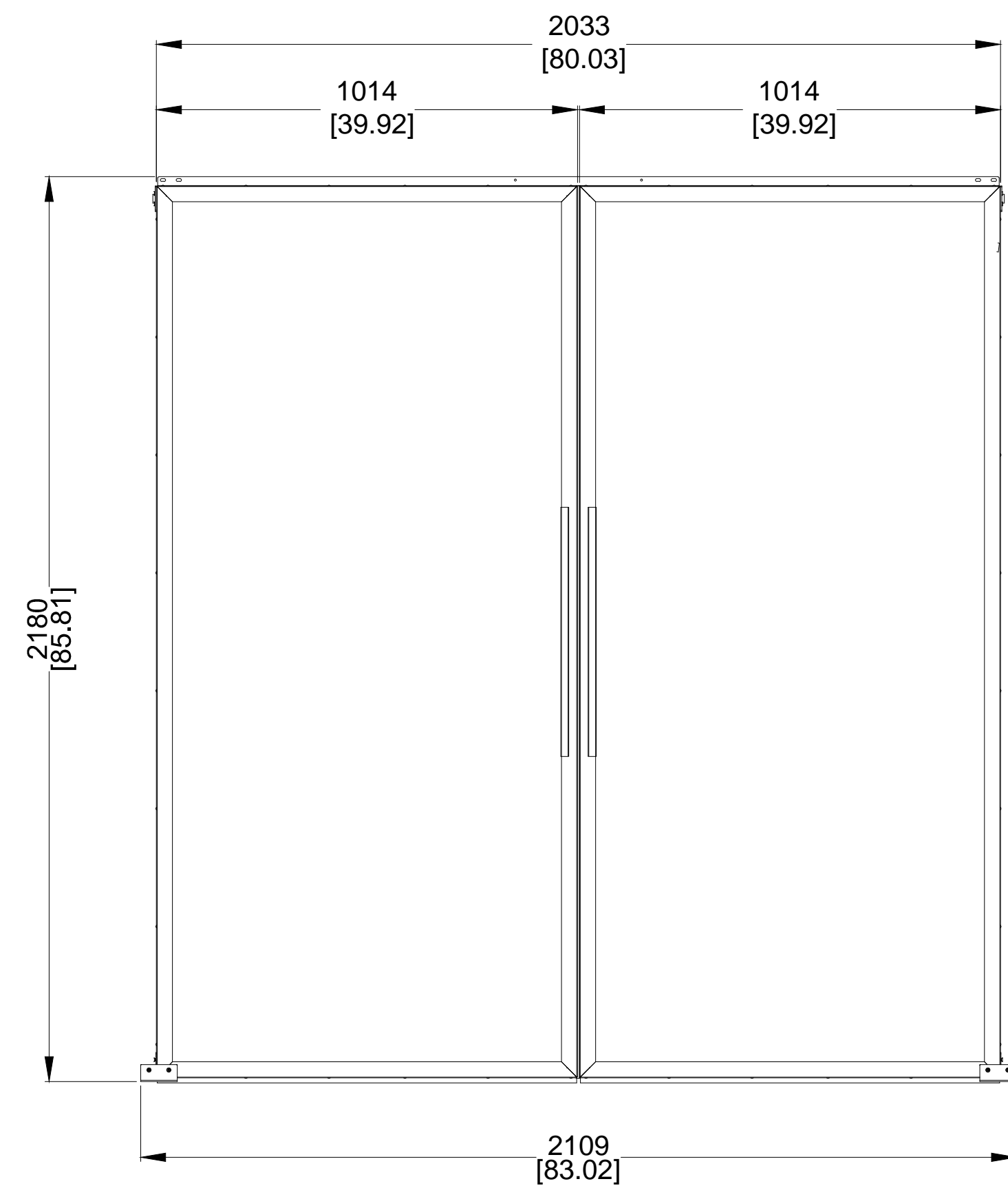
FRONT VIEW
