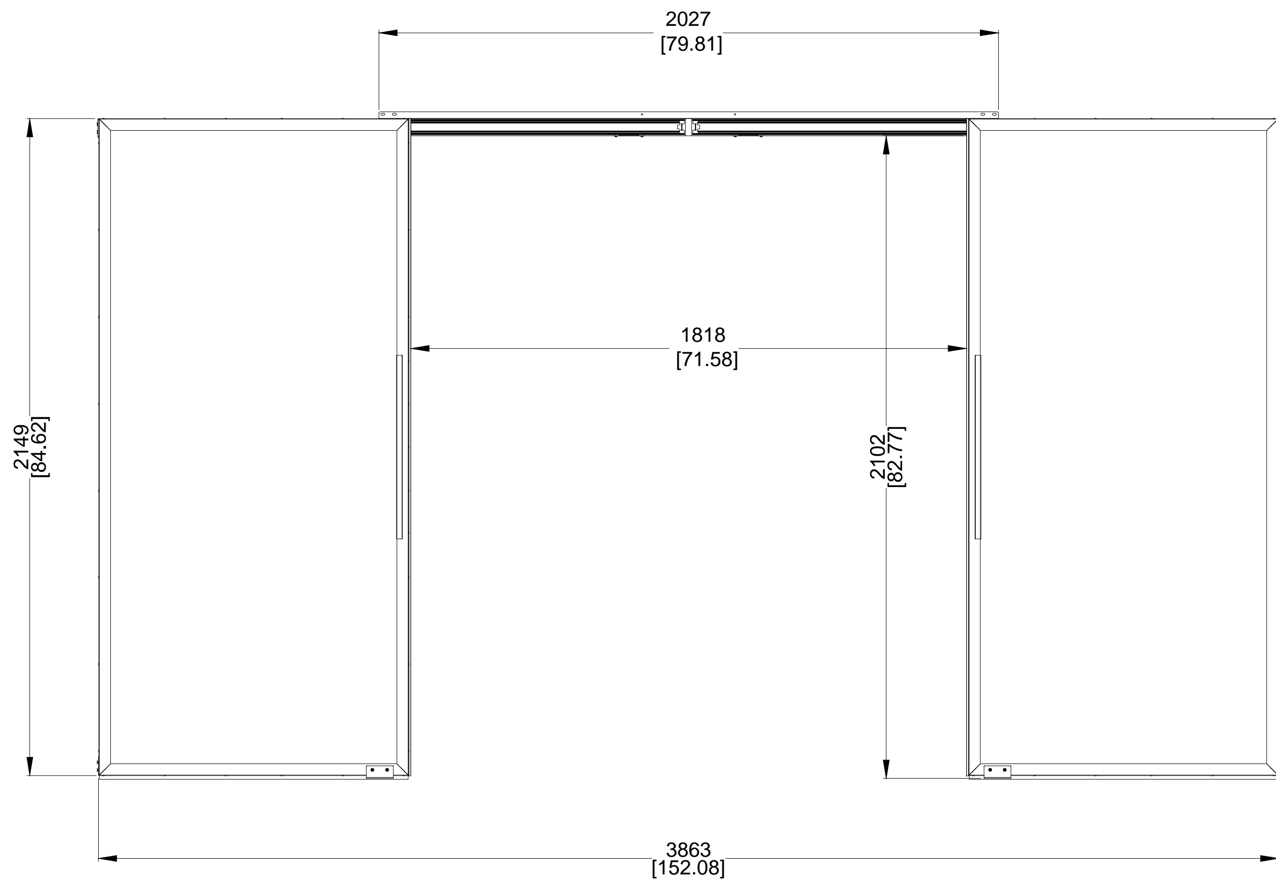
FRONT VIEW
