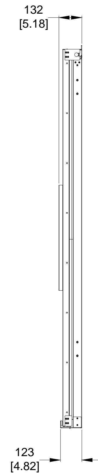
SIDE VIEW
