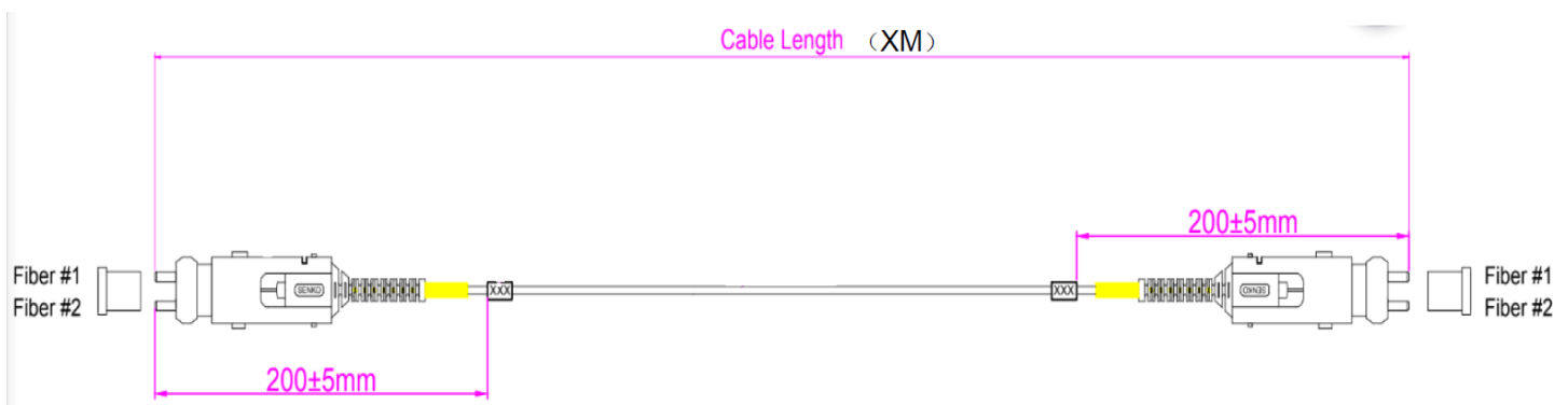
Figure 1 - SN-SN Uniboot Singlemode Fiber Optic Cable
