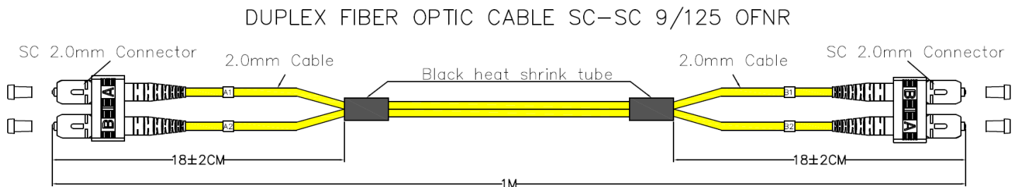
Figure 1 - SC-SC Duplex Singlemode Fiber Optic Cable
