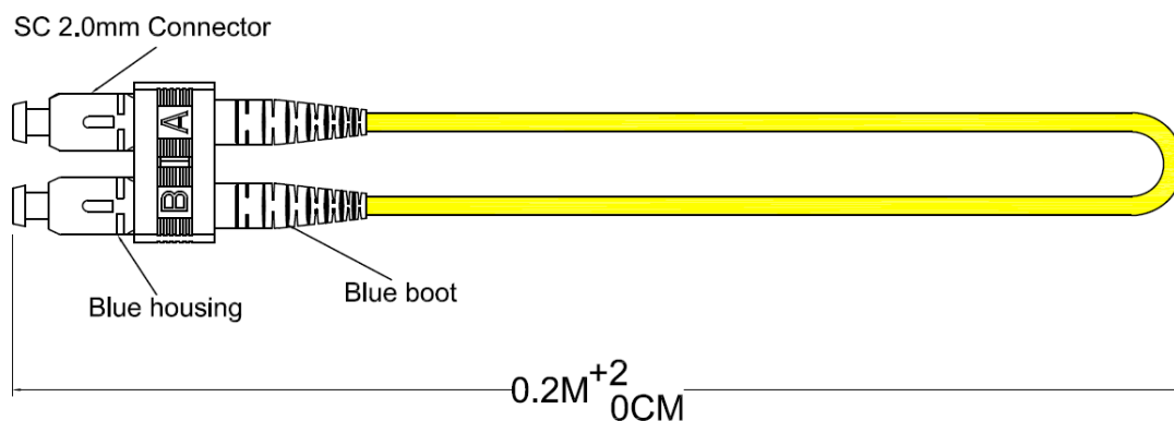
Figure 1 - SC-SC Singlemode Loopback Fiber Optic Cable
