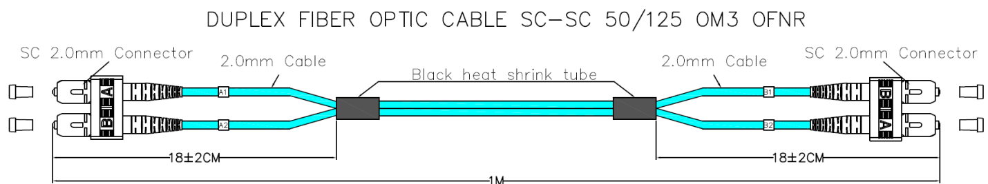
Figure 1 - SC-SC Duplex Multimode OM4 Fiber Optic Cable
