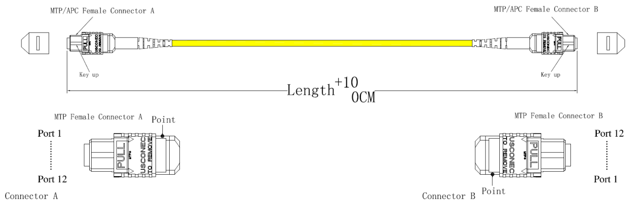
Figure 1 -MTP-MTP 12F Singlemode Fiber Optic Cable
