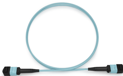
Figure 1 -MTP-MTP 24F Multimode OM3 Fiber Optic Cable
