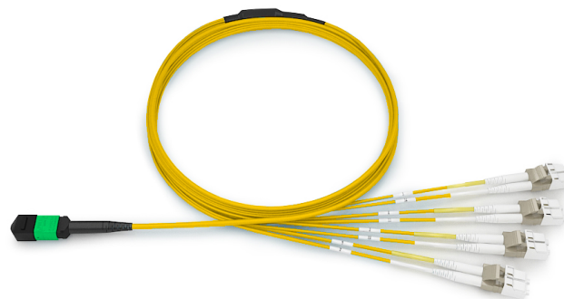
Figure 1 -MTP-LC 8F Singlemode Fiber Optic Cable
