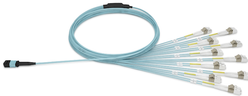
Figure 1 -MTP-LC 20F Multimode OM3 Fiber Optic Cable
