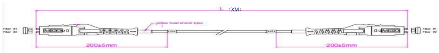
Figure 1 - MDC-MDC Uniboot Singlemode Fiber Optic Cable
