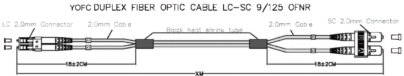
Figure 1 - LC-SC Duplex Multimode OM3 Fiber Optic Cable
