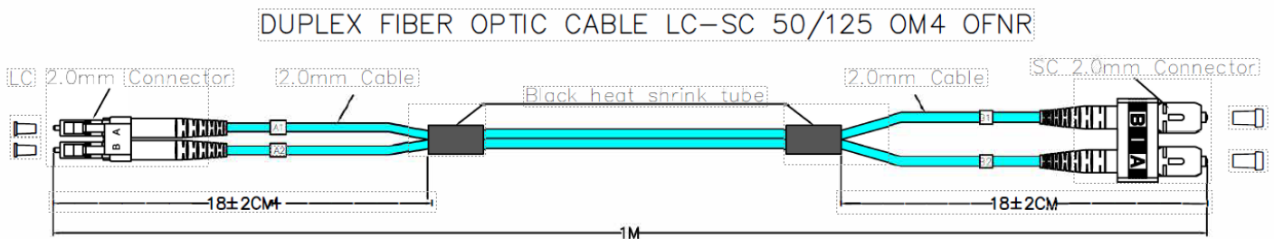
Figure 1 - LC-SC Duplex Multimode OM4 Fiber Optic Cable
