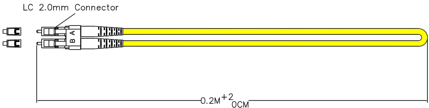
Figure 1 - LC-LC Singlemode Loopback Fiber Optic Cable
