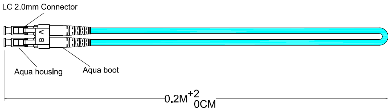
Figure 1 -LC-LC Loopback Multimode OM3 Fiber Optic Cable
