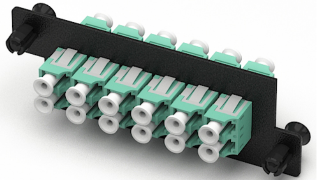
Figure 1: Multimode Passthrough Panel
