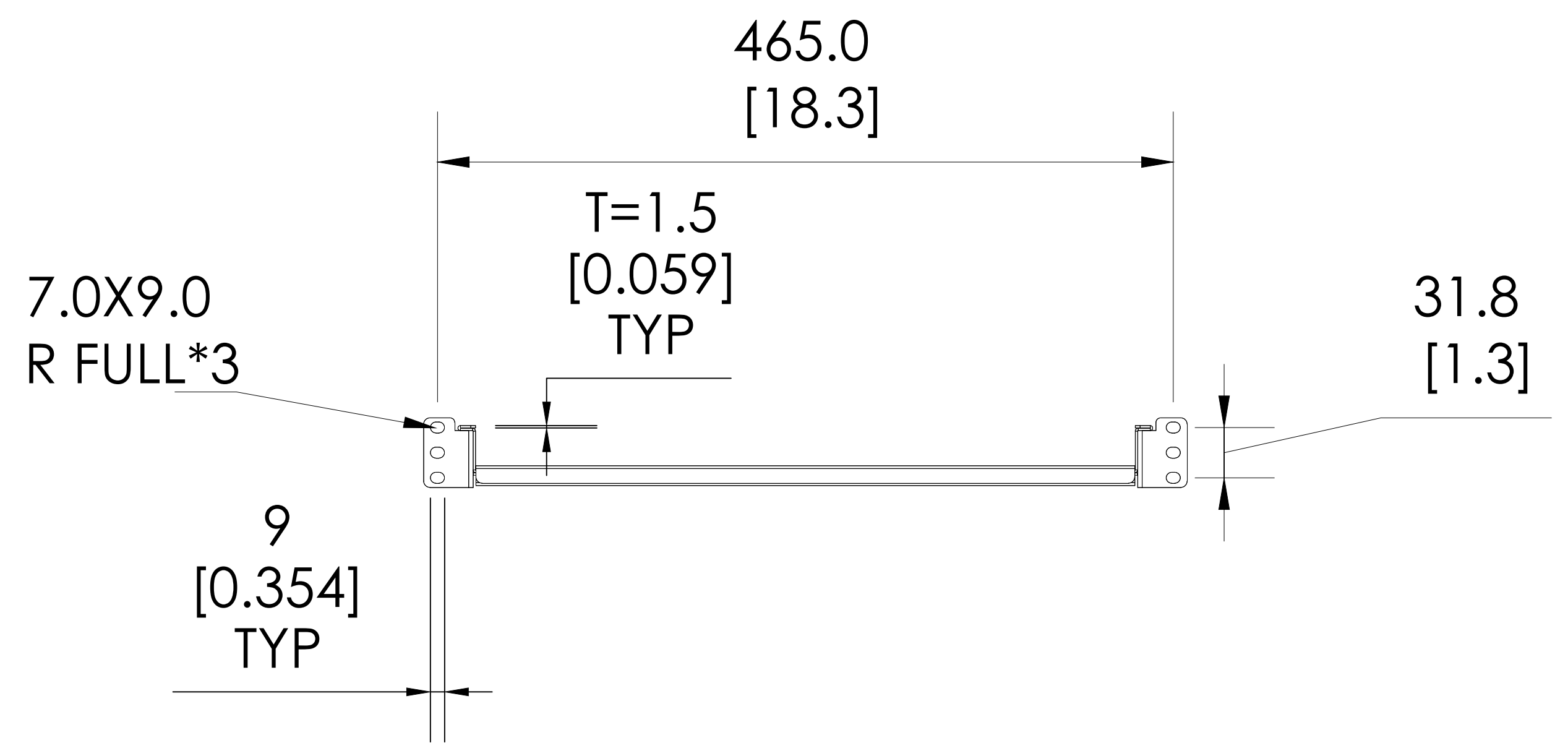
FRONT VIEW
