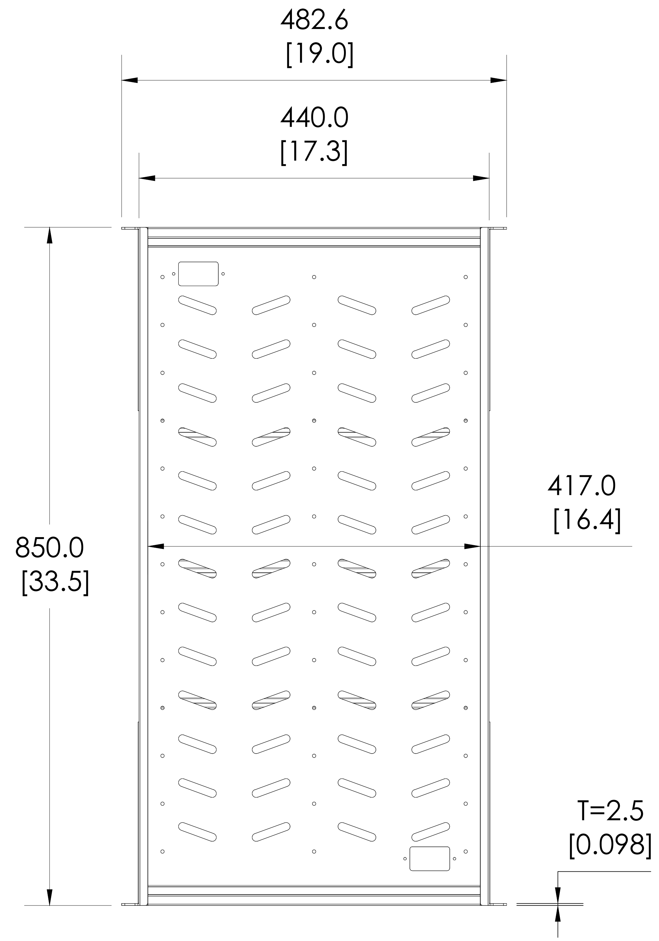
TOP VIEW
