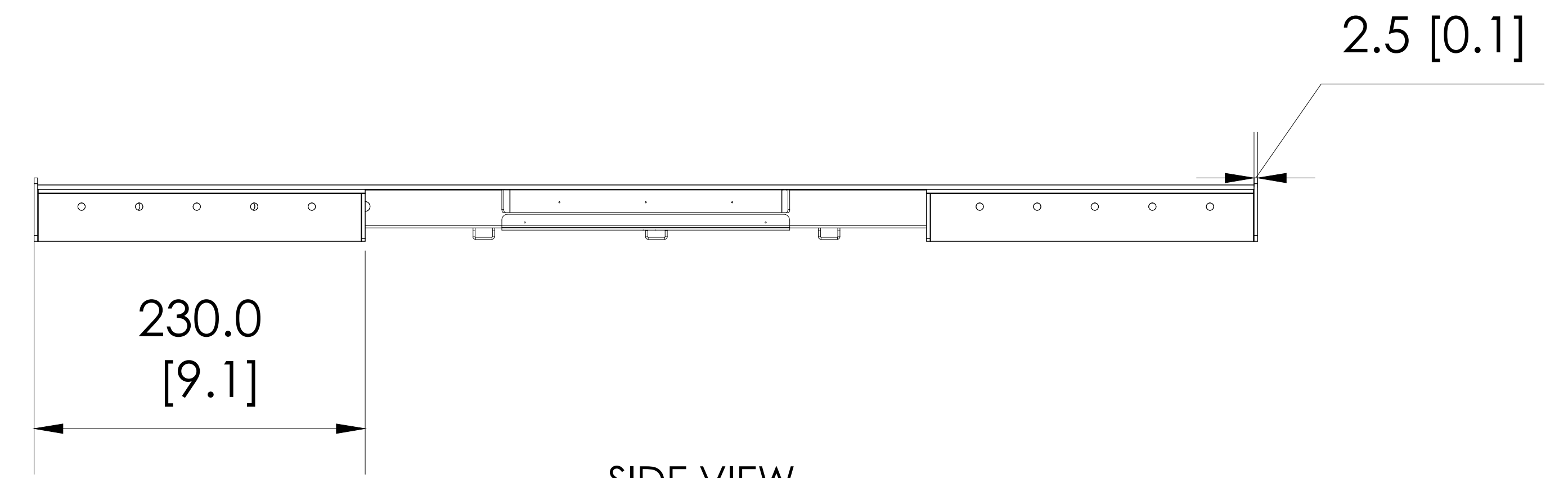
SIDE VIEW
