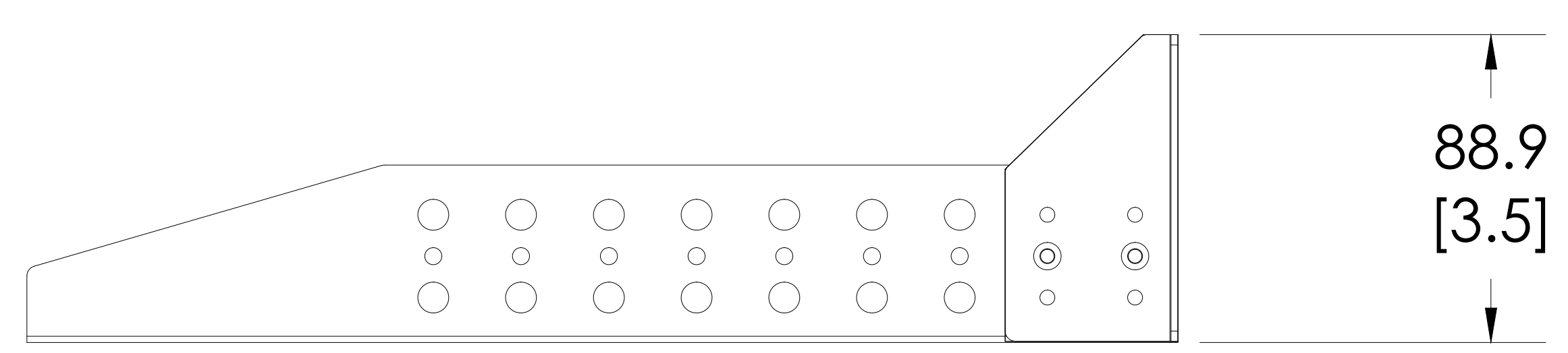
SIDE VIEW
