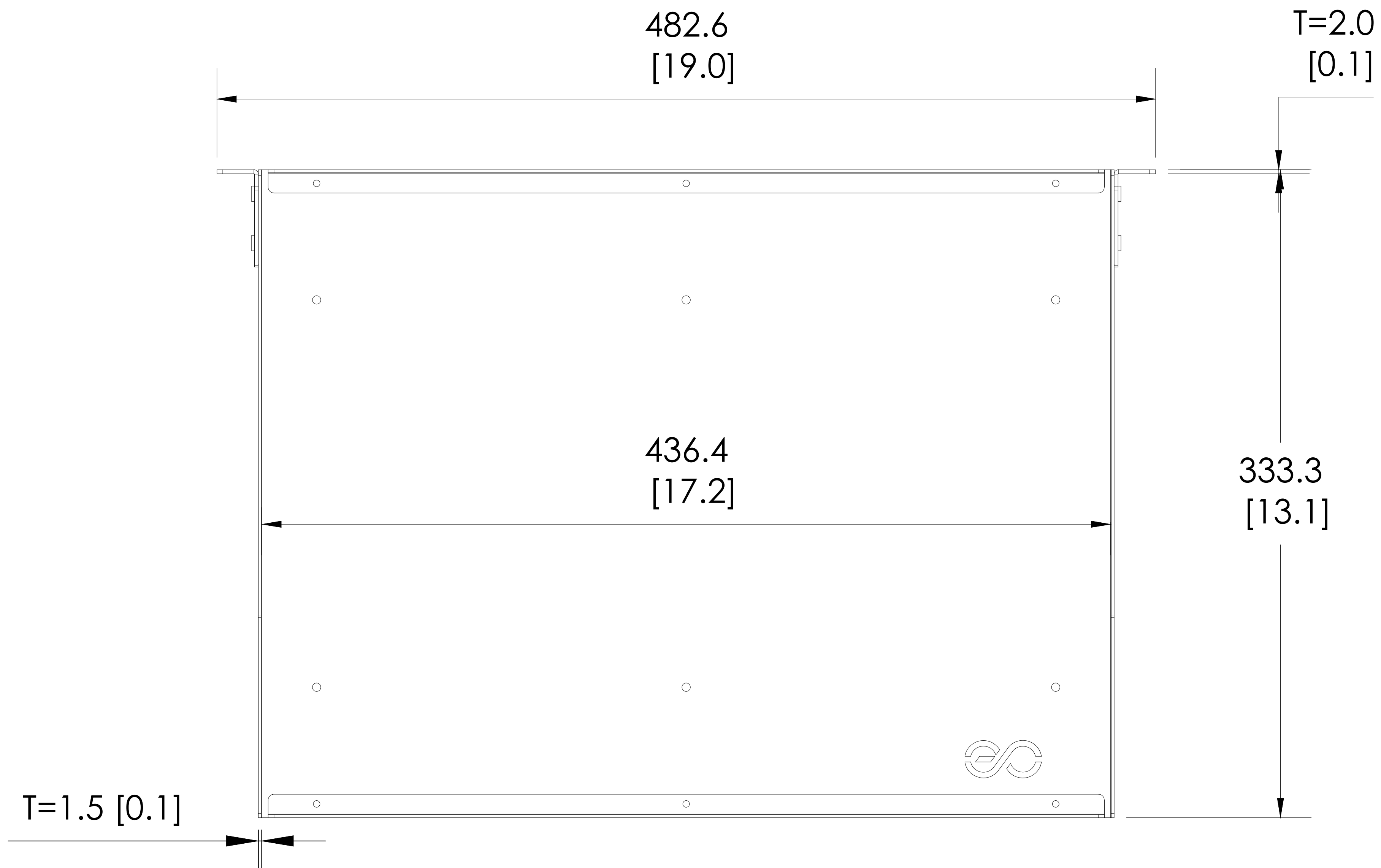
TOP VIEW
