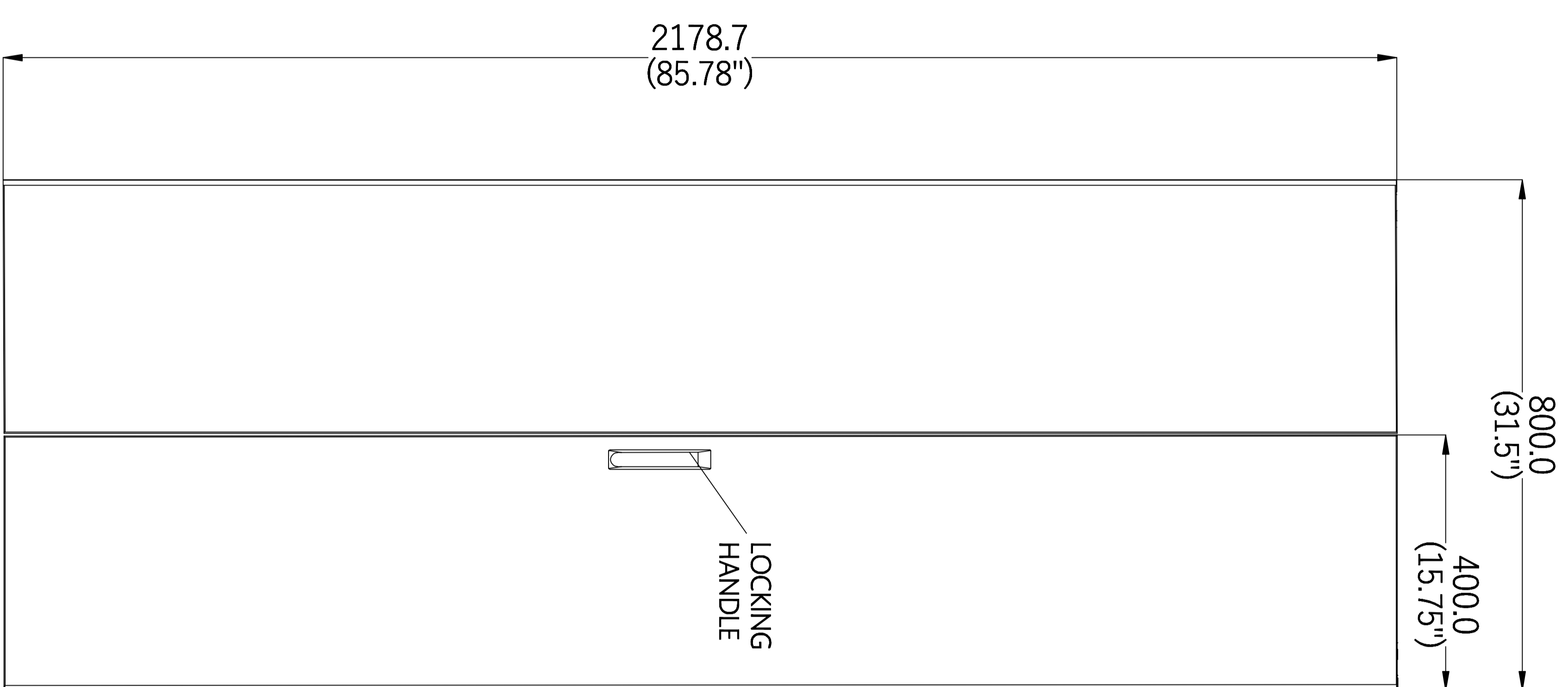
Rear Split Mesh Door
