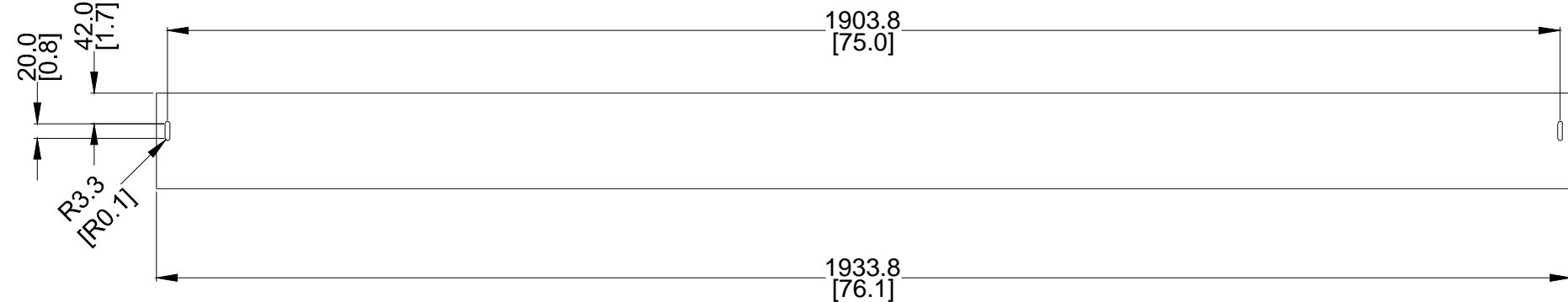
FRONT VIEW
