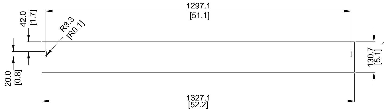
FRONT VIEW
