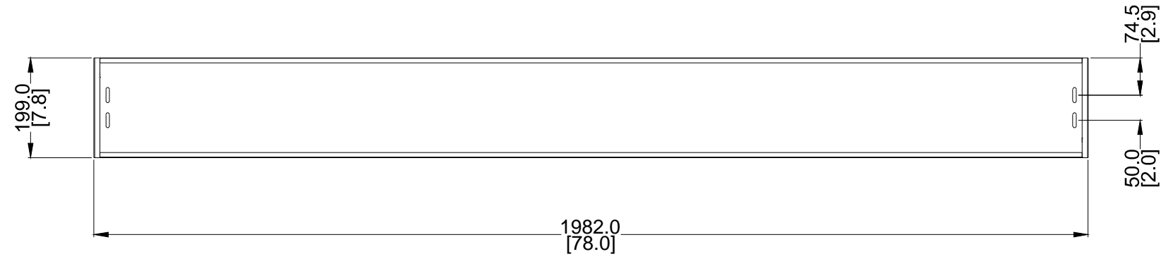
TOP VIEW
