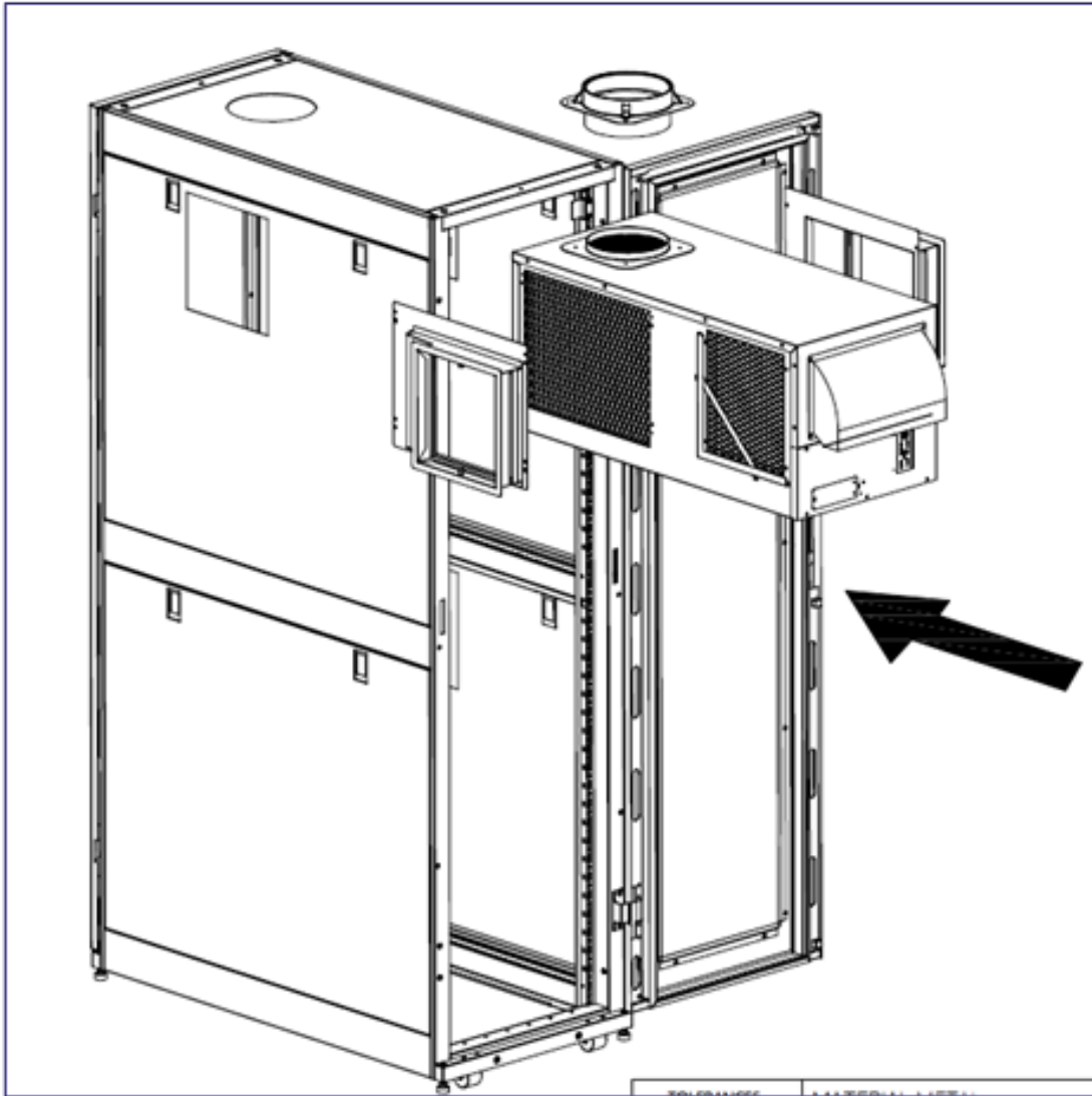
Figure 2 - EdgeRack RCU Installation Guide
