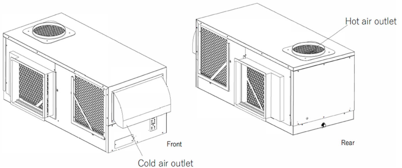
Figure 3 - Rack Cooling Unit
